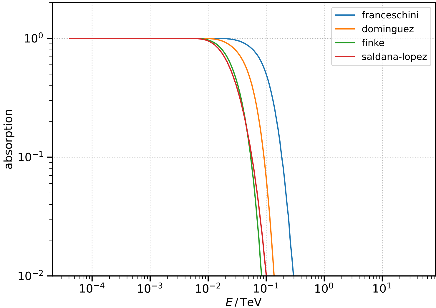
EBL absorption at z=1
